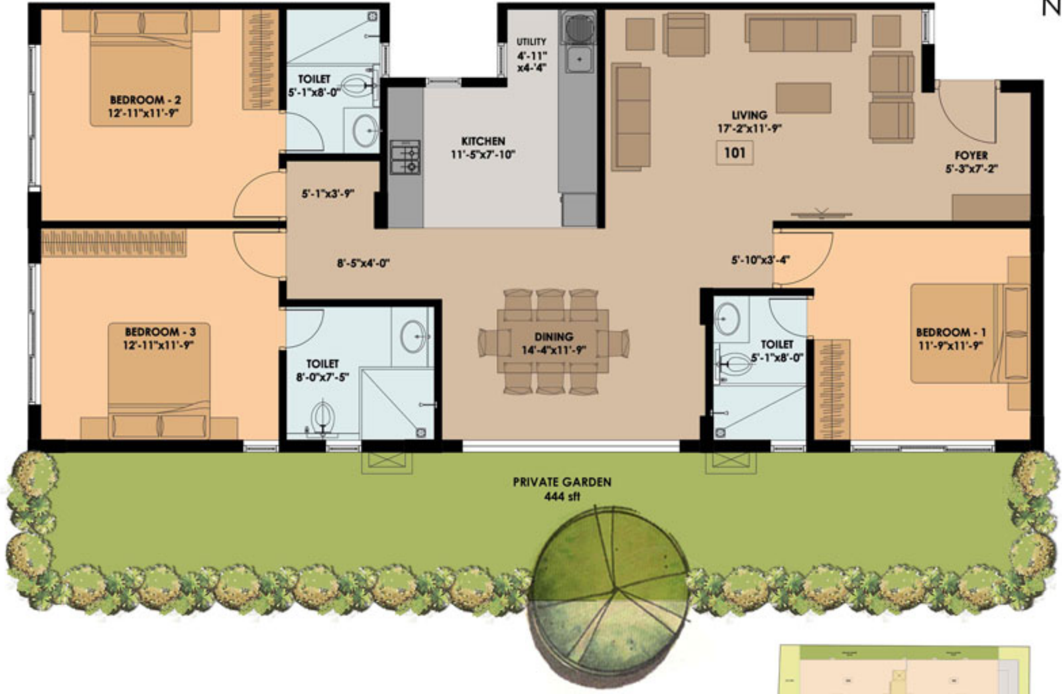
101- GROUND FLOOR PLAN UDYAAN 2- FOR GRIHA PROMOTERS PVT. LTD.
